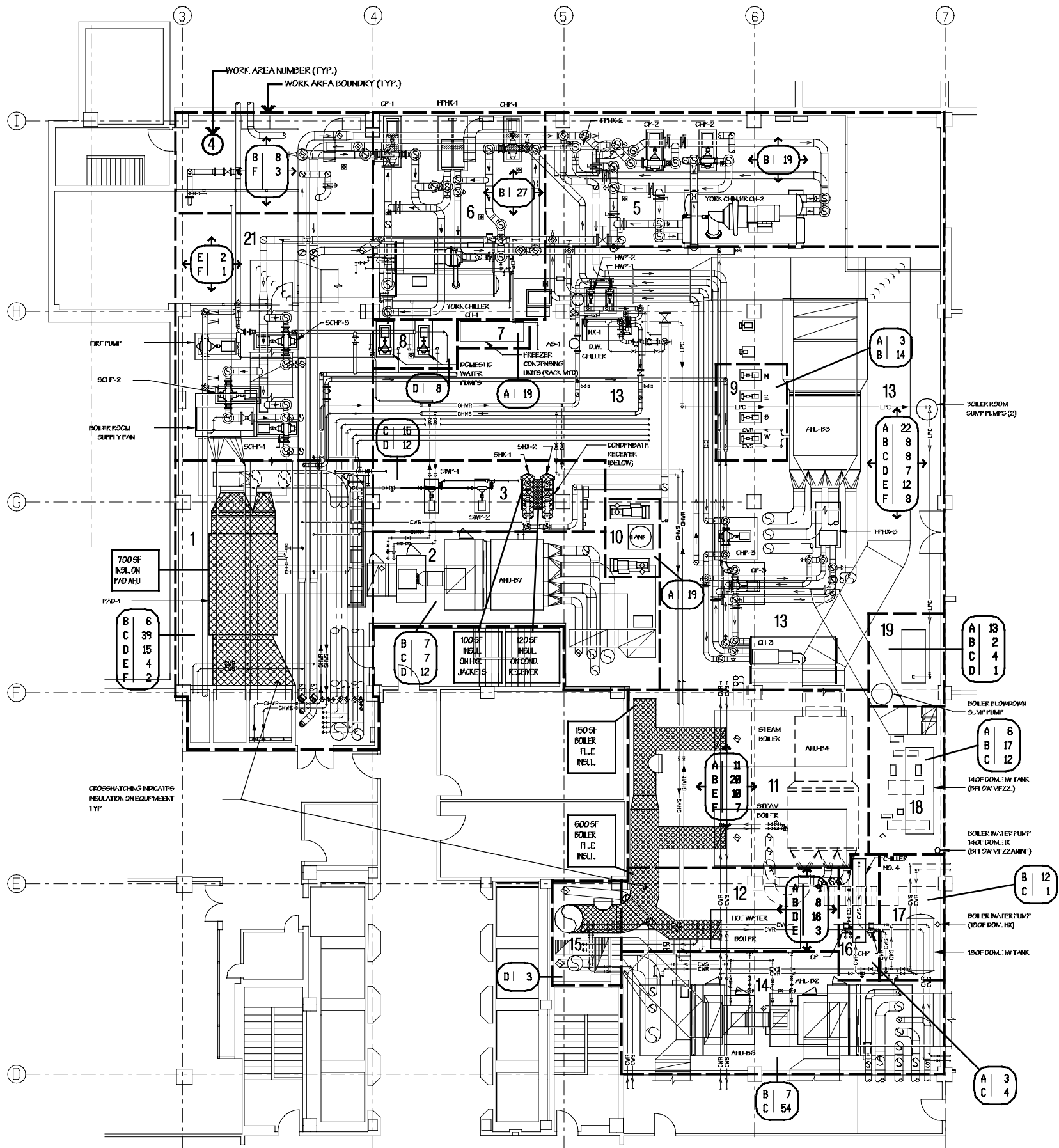
1 MAIN MECHANICAL ROOM SUB-BASEMENT FLOOR PLAN ASBESTOS ABATEMENT SCALE: 1/8" = 1'-0"
