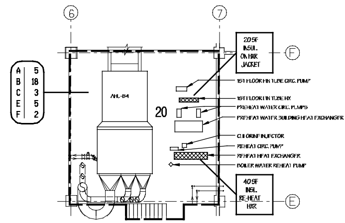
2 SUB-BASEMENT MEZZANINE FLOOR PLAN SCALE: 1/8" = 1'-0"
